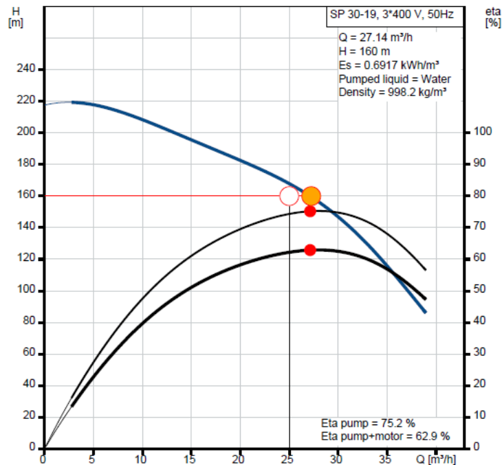
Figure 4-9; Variable speed performance curve of the pump selected for Kiwenda Water System
