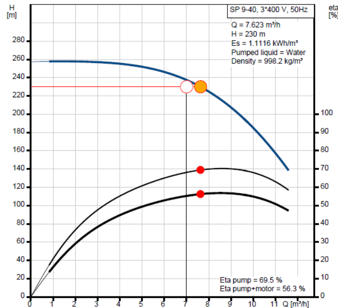
Figure 4-1; Variable speed performance curve of the pump selected for Bamunanika Water System
