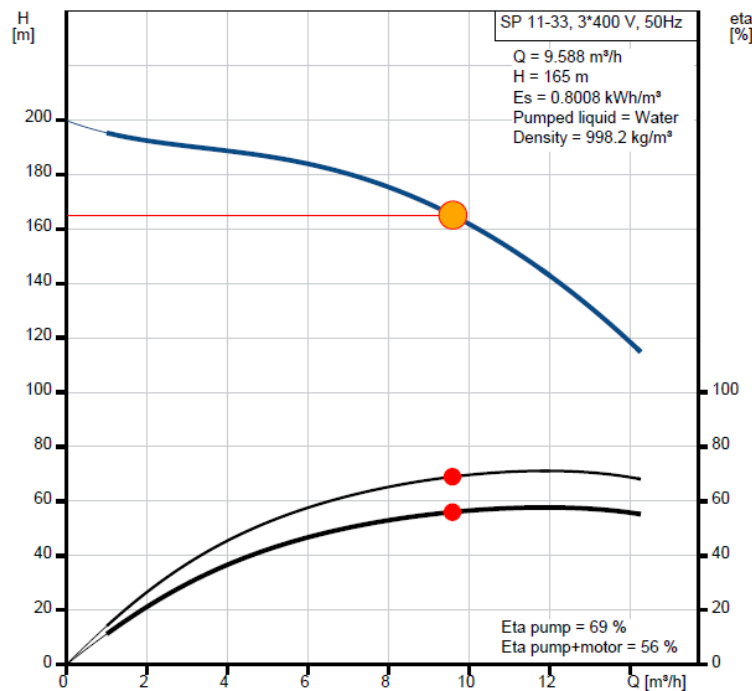
Figure 4-17; Variable speed performance curve of the pump selected for Kagulu Water System
