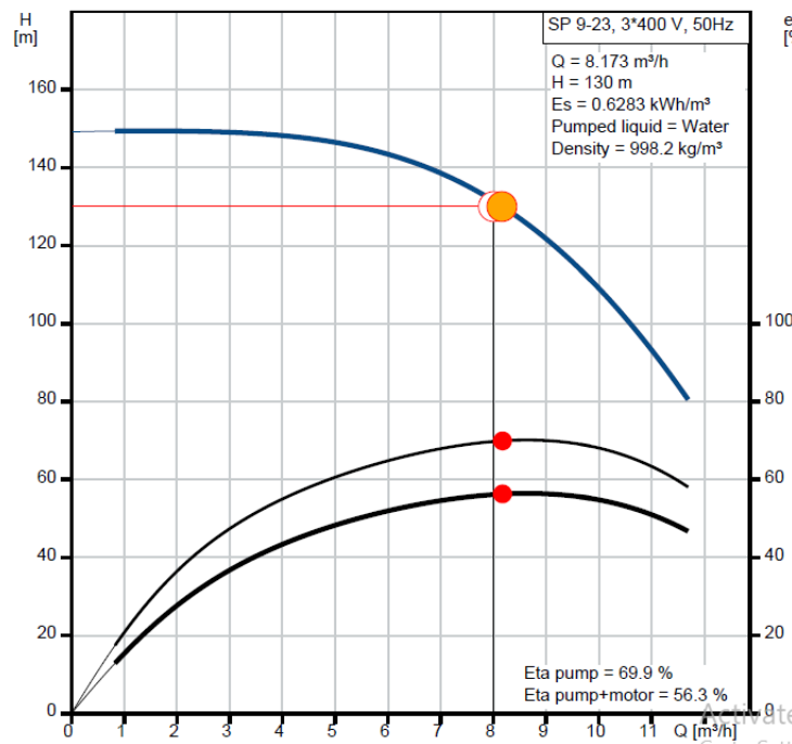
Figure 4-19; Variable speed performance curve of the pump selected for Kasambira Water System
