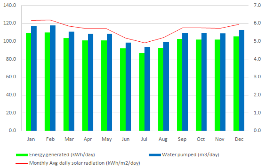
Figure 4-12; Daily Water pumping performance of the Mayanga energy package
