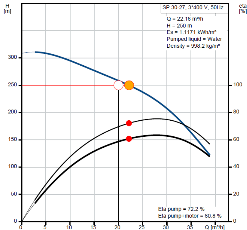
Figure 4-7; Variable speed performance curve of the pump selected for Kikyusa Water System
