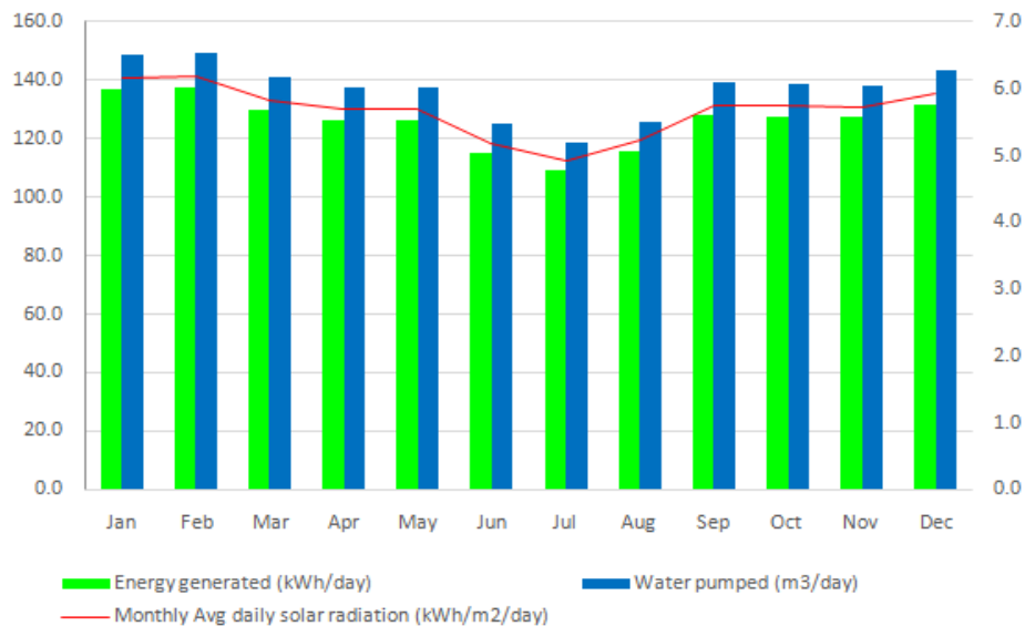
Figure 4-10; Daily Water pumping performance of the Kiwenda energy package
