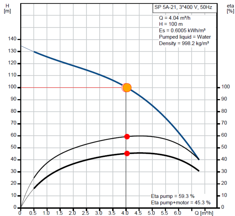
Figure 4-3; Variable speed performance curve of the pump selected for Banda Water System
