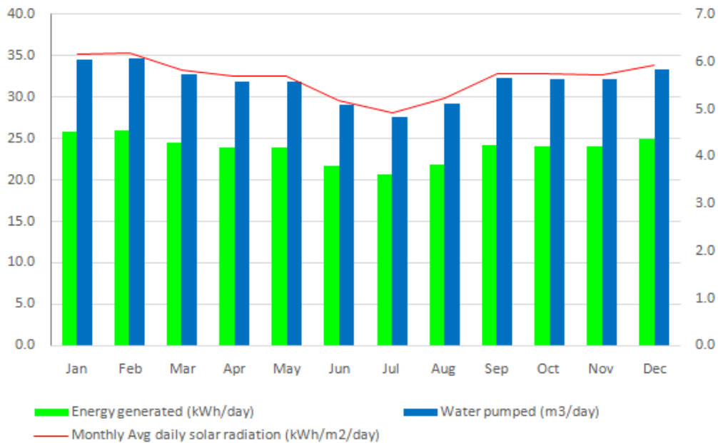
Figure 4-16; Daily Water pumping performance of the Buyende-2 energy package
