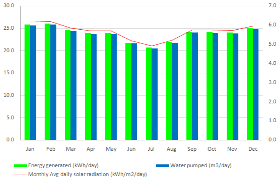
Figure 4-4; Daily Water pumping performance of the Banda energy package
