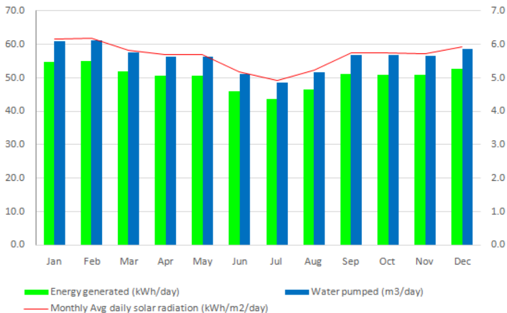
Figure 4-20; Daily Water pumping performance of the Kasambira energy package
