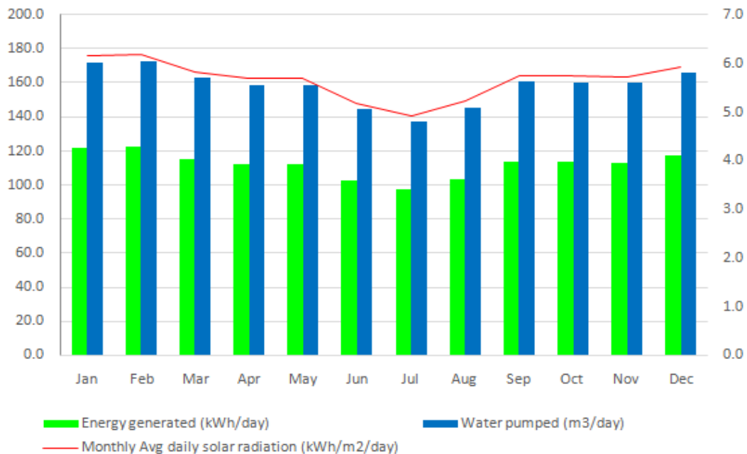
Figure 4-6; Daily Water pumping performance of the Kayunga energy package
