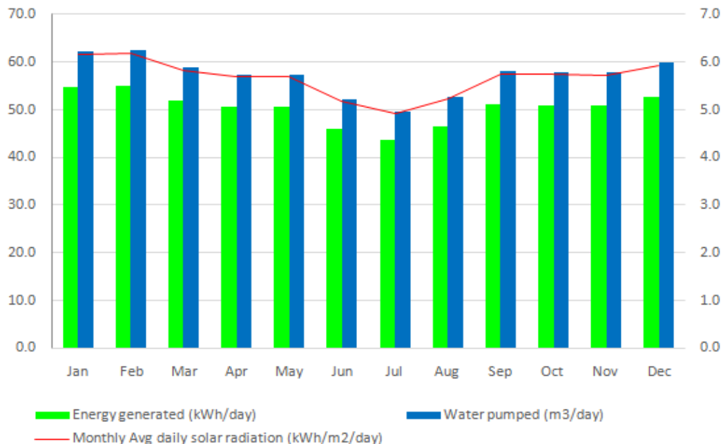
Figure 4-14; Daily Water pumping performance of the Ssekanyonyi energy package
