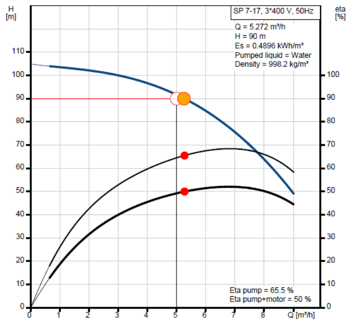
Figure 4-15; Variable speed performance curve of the pump selected for Buyende-2 Water System
