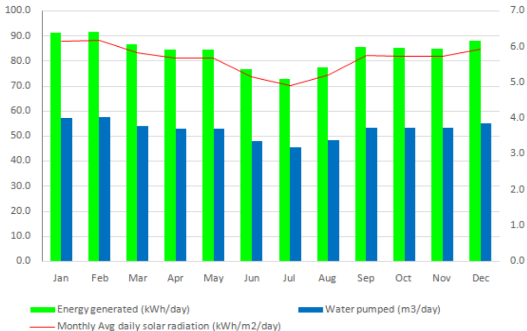
Figure 4-2; Daily Water pumping performance of the Bamunanika energy package
