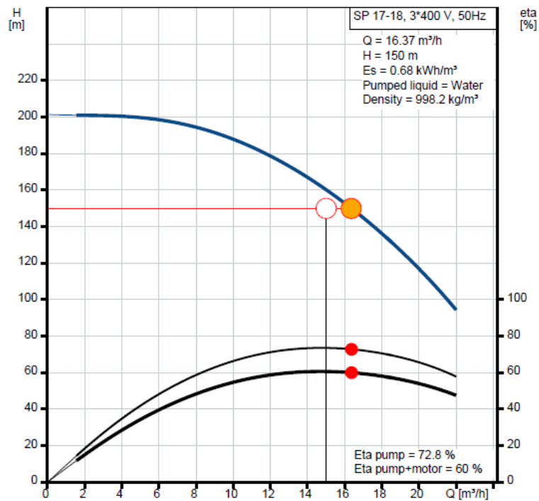
Figure 4-11; Variable speed performance curve of the pump selected for Mayanga Water System
