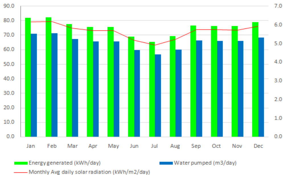
Figure 4-18; Daily Water pumping performance of the Kagulu energy package
