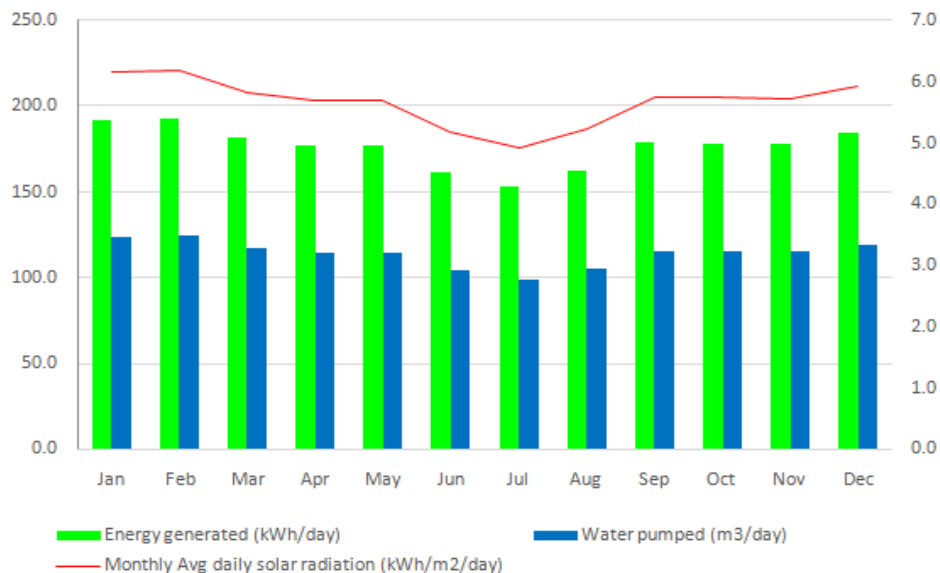
Figure 4-8; Daily Water pumping performance of the Kikyusa energy package
