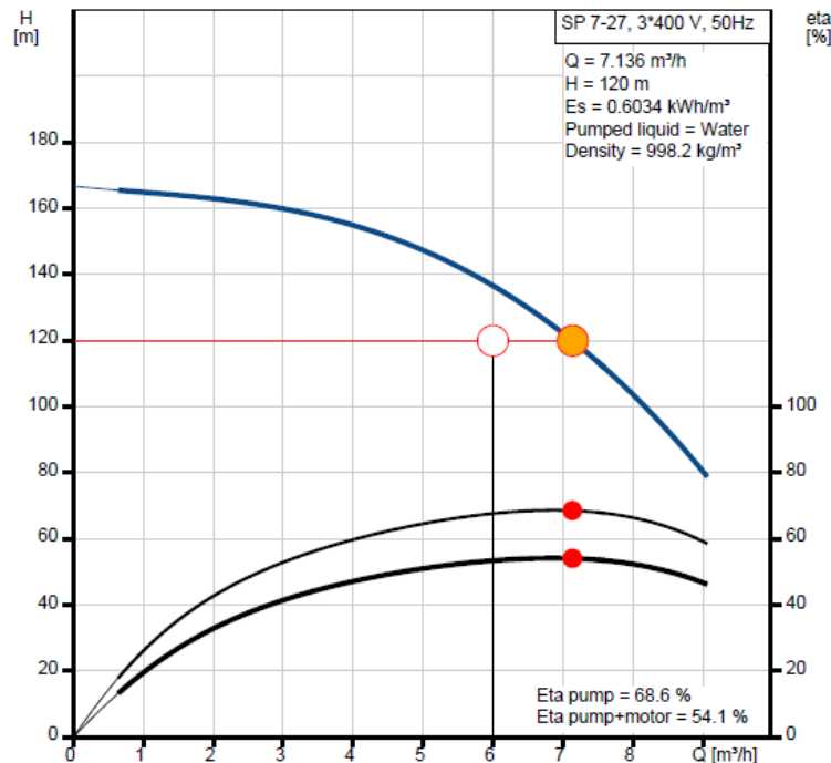
Figure 4-13; Variable speed performance curve of the pump selected for Ssekanyonyi Water System
