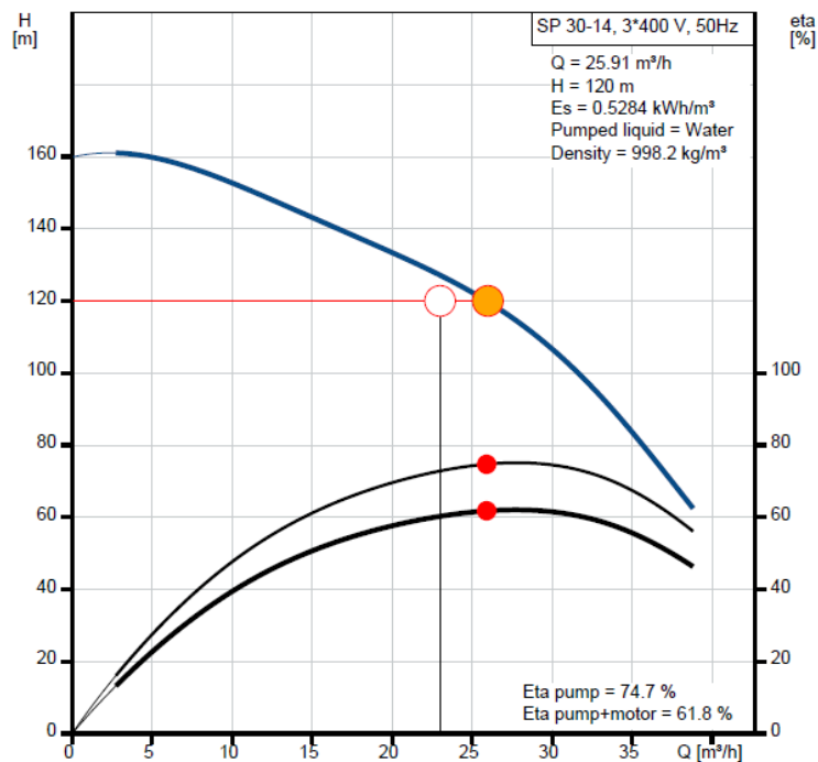
Figure 4-5; Variable speed performance curve of the pump selected for Kayunga Water System
