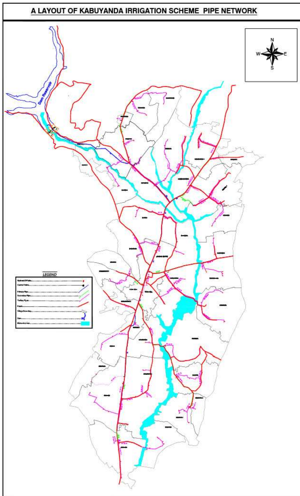
Figure 1: A layout of Kabuyanda Irrigation Scheme Pipe Network
