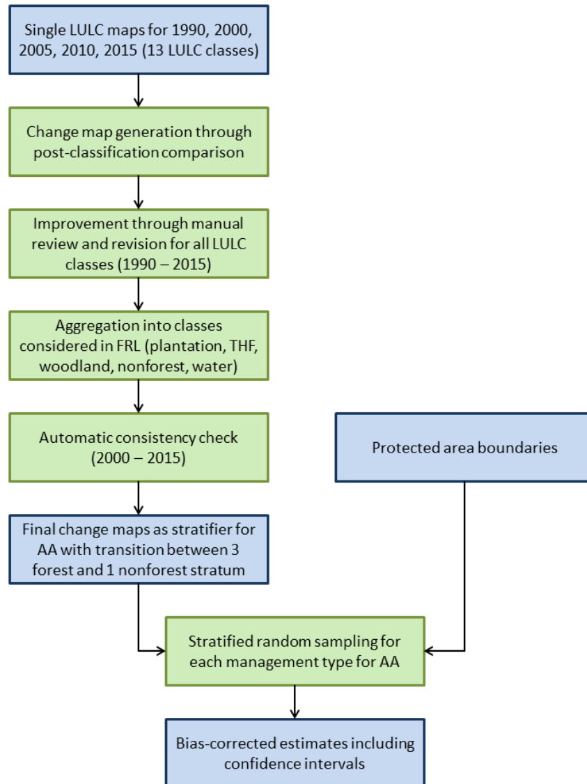
Figure 4: Work flow for creation of change maps and bias-corrected estimates.
